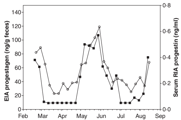
Fig. 4. Comparison of hormone profiles from an adult female African elephants. Profiles were generated from faeces (○) using 70% propanol and a precoated EIA microtitre plates stored for 1 month at room temperature, and from serum (■) using a solid-phase ^{125}\text{I} RIA.
