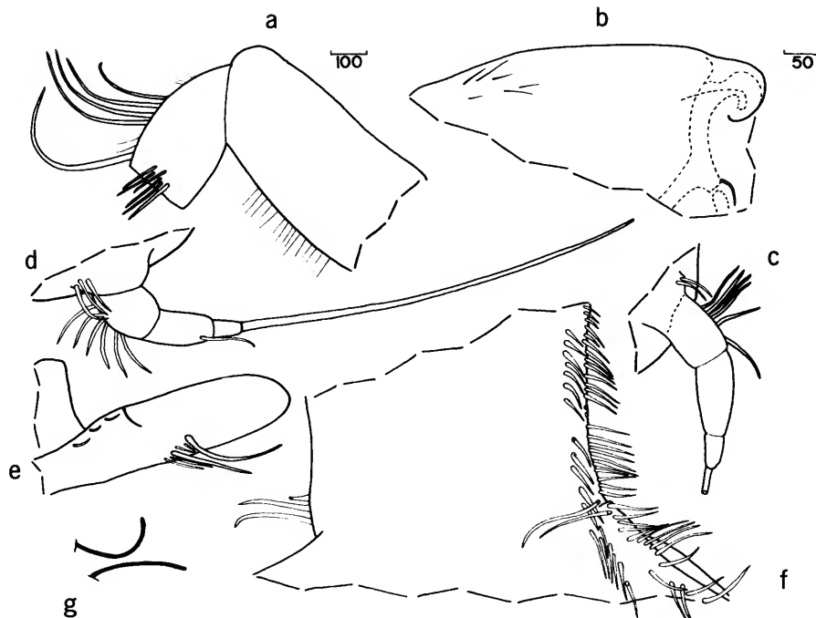
FIGURE 12.— Cycloleberis galathea Poulsen, holotype, A-1 female: a , joints 1 and 2 of left 1st antenna, lateral view; b , distal end of protopodite of left 2nd antenna, medial view; c , endopodite of left 2nd antenna, medial view; d , endopodite of right 2nd antenna, medial view; e , comb of right 5th limb (small exopodial bristles obscure, hairs and ventral bristles not shown); f , proximal part of left 6th limb, medial view; g , segmented strands of foreign growth on dorsal margin of protopodite of left 2nd antenna, medial view. (Same magnification in micrometers: a,e ; b-d,f,g .)
