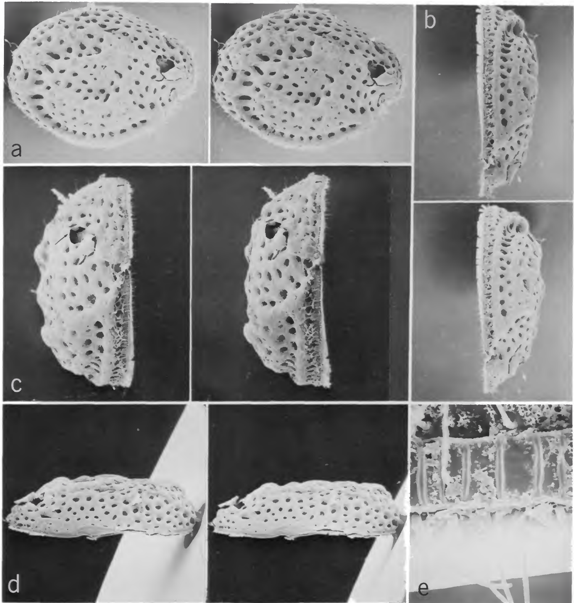
FIGURE 21.— Astropterion setiferum Kornicker and Caraion, variety B, adult female, USNM 149285, right valve (cleaned in sonic vibrator): a , lateral view, stereo pair, \times 38 ; b , ventral view, stereo pair, anterior to left, \times 40 ; c , anterior view, stereo pair, \times 55 ; d , dorsal view, stereo pair, anterior to left, \times 38 ; e , detail, from b , showing ventral edge of valve (broad white band in photograph is the lamellar prolongation of the selvage), lateral view, \times 1000 . (Photos reduced to 70 percent for publication.)
