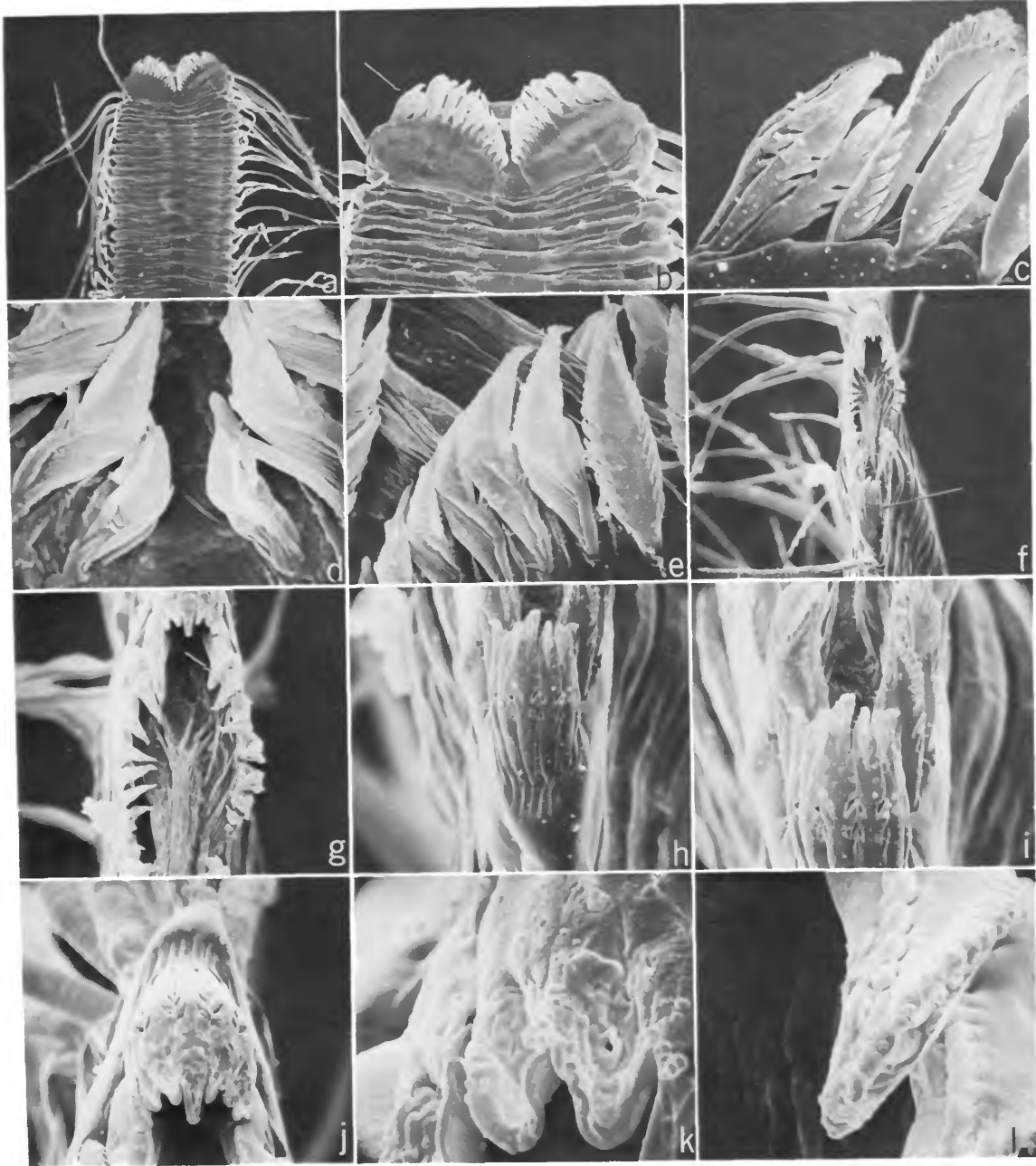
FIGURE 7.— Cycloleberis squamiger (Scott), adult female, USNM 149278A, 7th limb: a, distal part, \times 200 ; b, tip of limb shown in a, \times 500 ; c, comb bristles shown in b (for location see left arrow in b) \times 2700 ; d, midbristles in b, \times 5000 ; e, bristles to right of middle in b, \times 3000 ; f, end view of limb, \times 500 ; g, same, \times 1230 ; h, bristles forming lower comb shown in f (see arrow in f), \times 1790 ; i, same, \times 2465 ; j, bristles forming upper comb shown in f, \times 2465 ; k, bristles on left end of comb shown in j, note pore, \times 11,000 ; l, tip of midbristles of comb (for location see arrow in g), \times 8830 . (Photos reduced to 54 percent for publication.)
