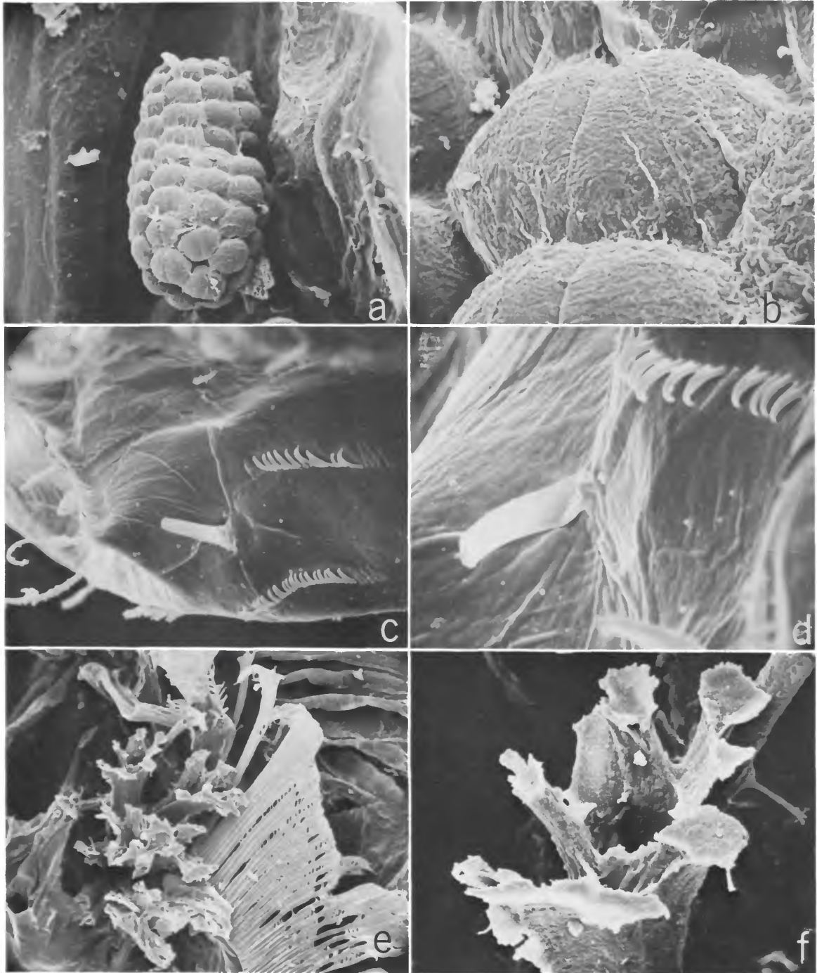
FIGURE 9.— Cycloleberis squamiger (Scott), adult female, USNM 149278A: a , left lateral eye, \times 240 ; b , detail of ommatidia in a , \times 2000 ; c , part of upper lip, \times 2415 ; d , part of upper lip, \times 6040 ; e , left end of central adductor muscles, anterior to left, \times 125 ; f , detail of e , \times 500 . (Photos reduced to 82 percent for publication.)
