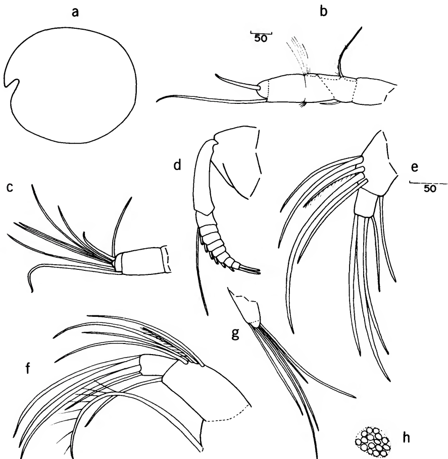
FIGURE 10.— Cycloleberis squamiger (Scott), lectotype, juvenile: a, outline of specimen, length 1.09 mm; b, left 1st antenna, lateral view (only a-claw of end joints shown); c, end of right 1st antenna, medial view; d, part of protopodite and exopodite of left 2nd antenna (only proximal parts of exopodial bristles shown); e, tip of right mandible, medial view; f, distal part of left mandible, lateral view; g, tip of left maxilla, medial view; h, left lateral eye, anterior to left. (Specimen not dissected; appendages drawn were either protruding from shell or visible through shell. Same magnification in micrometers: b-d,g,h; e,f.)
