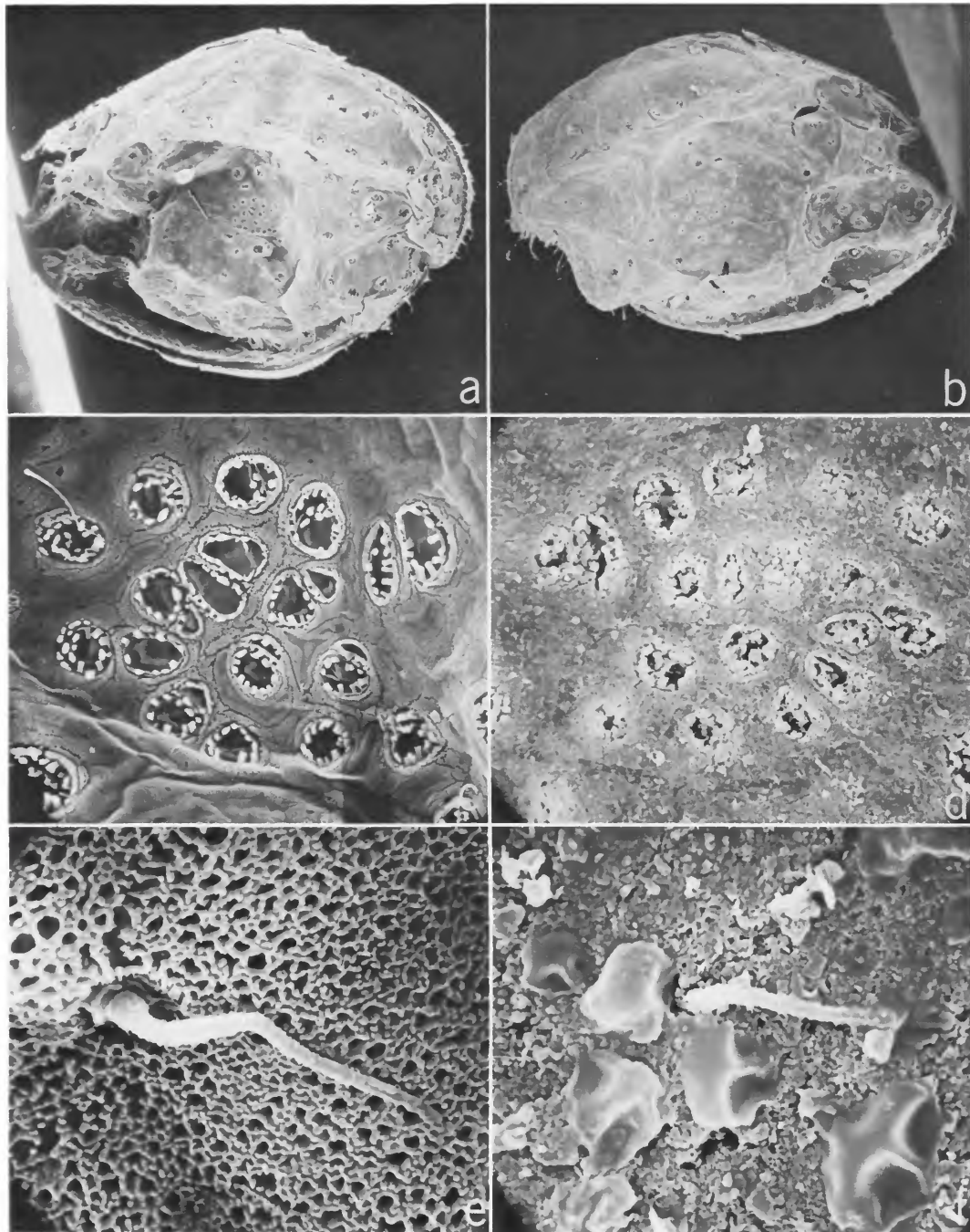
FIGURE 15.— Asteropteron setiferum variety A, adult female, USNM 143996, comparison of valves treated and untreated with sonic vibrator: a , right valve (cleaned with sonic vibrator), \times 42 ; b , left valve (not cleaned), \times 42 ; c , detail, from a , of fossae in vicinity of central muscle scars, \times 340 ; d , same, from b , \times 340 ; e , detail, from a , of hair and surface textures between fossae, \times 5000 ; f , same, from b , \times 5000 . (Photos reduced to 75 percent for publication.)
