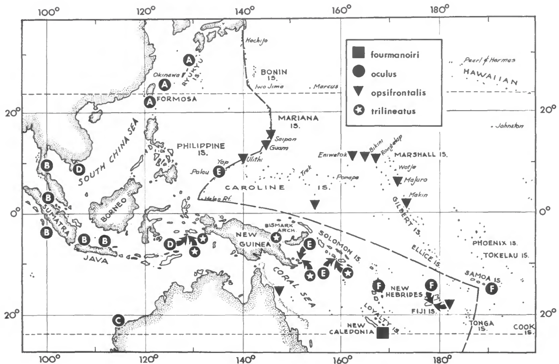
FIGURE 7.—Distribution of the Ecsenius oculus subgroup; the 6 color pattern types (A-F) of E. oculus indicated. (Irregular broken line indicates approximate position of Andesite Line.)
