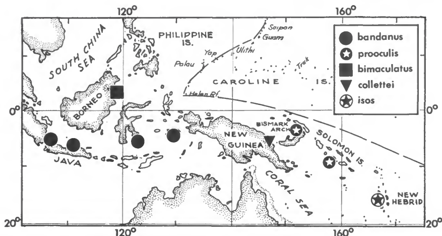
FIGURE 2.—Distribution of the species of the Ecsenius prooculis subgroup. (Irregular broken line indicates approximate position of Andesite Line.)
