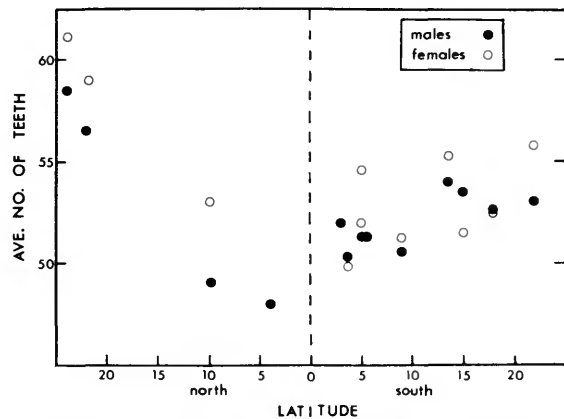
FIGURE 8.—Variation in mean numbers of dentary incisor teeth of Ecsenius oculus as correlated with latitude (based on data in Table 9).
