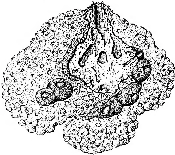
FIGURE 2.— Montastrea annularis infested by Siphonodictyon cachacrouense , new species. Part of the coral is removed to show the internal structure of the sponge (0.6 ×).
