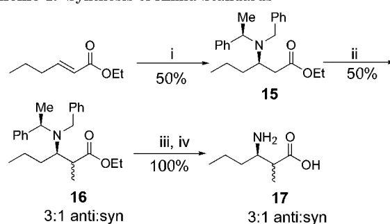
Scheme 1. Synthesis of Amha Standards a
