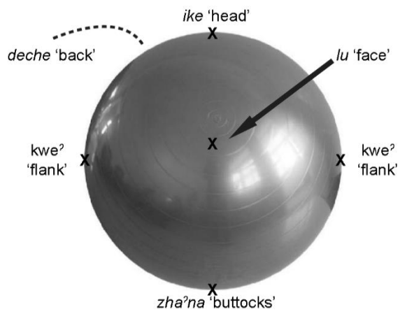
Figure 4. BPTs mapped onto a ball
