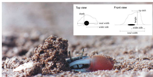
Fig. 1. A male fiddler crab ( Uca uruguayensis ) with a hood. Illustrations within the box show the measurements made on hoods. This figure is published in colour in the online edition of this journal, which can be accessed via http://booksandjournals.brillonline.com/content/journals/1937240x .
