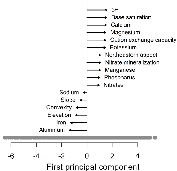
(b) PCA for sapling recruitment ( 20 \times 20 m scale)
