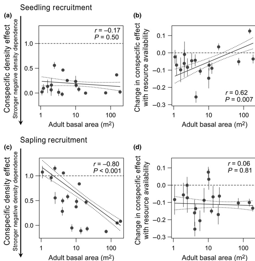
Figure 4 The relative strength of conspecific negative density dependence (CNDD) and changes in the strength of CNDD with resource availability among common and rare species. (a) Strength of CNDD during seedling recruitment as a function of size-weighted abundance, measured as adult basal area (m 2 ). (b) The change in seedling CNDD with a 1 SD change in the soil-resource gradient (PC1) as a function of adult basal area. (c) Strength of CNDD during sapling recruitment as a function of adult basal area. (d) The change in sapling CNDD with a 1 SD change in the soil-resource gradient (PC1) as a function of adult basal area. Note that adult size-weighted abundance is plotted on a log scale.
