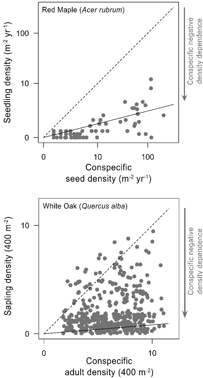
Figure S2. Plots showing seedling and sapling densities against conspecific seed and adult densities for red maple ( Acer rubrum ) and white oak ( Quercus alba ), respectively, in the Tyson Research Center Forest Plot, St. Louis, Missouri, USA. The strength of conspecific negative density dependence was measured as the slopes of these relationships after controlling for heterospecific density effects, with more negative slopes indicating conspecific negative density dependence (see Table S1, S2). The dashed line indicates a 1:1 relationship, which would be expected in the absence of conspecific negative density dependence. These methods are identical to those in Harms (2000), but we account for potential heterospecific density effects and test for interactions between woody-plant densities and the soil-resource gradient.
