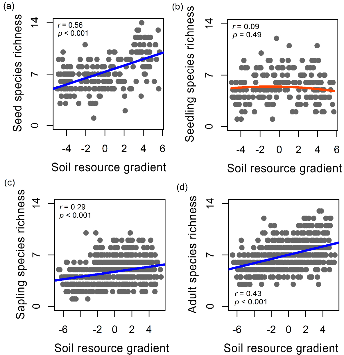
Figure S6. Changes in species richness for (a) seeds, (b) seedlings, (c) saplings, (d) and adults along the soil-resource gradient. Changes in rarefied richness along the soil-resource gradient were similar for the seed ( r = 0.22 ; p = 0.007 ), seedling ( r = 0.13 ; p = 0.20 ), sapling ( r = 0.16 ; p = 0.012 ), and adult ( r = 0.26 ; p < 0.001 ) life stages.
