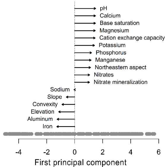
(a) PCA for seedling recruitment ( 10 \times 10 m scale)
