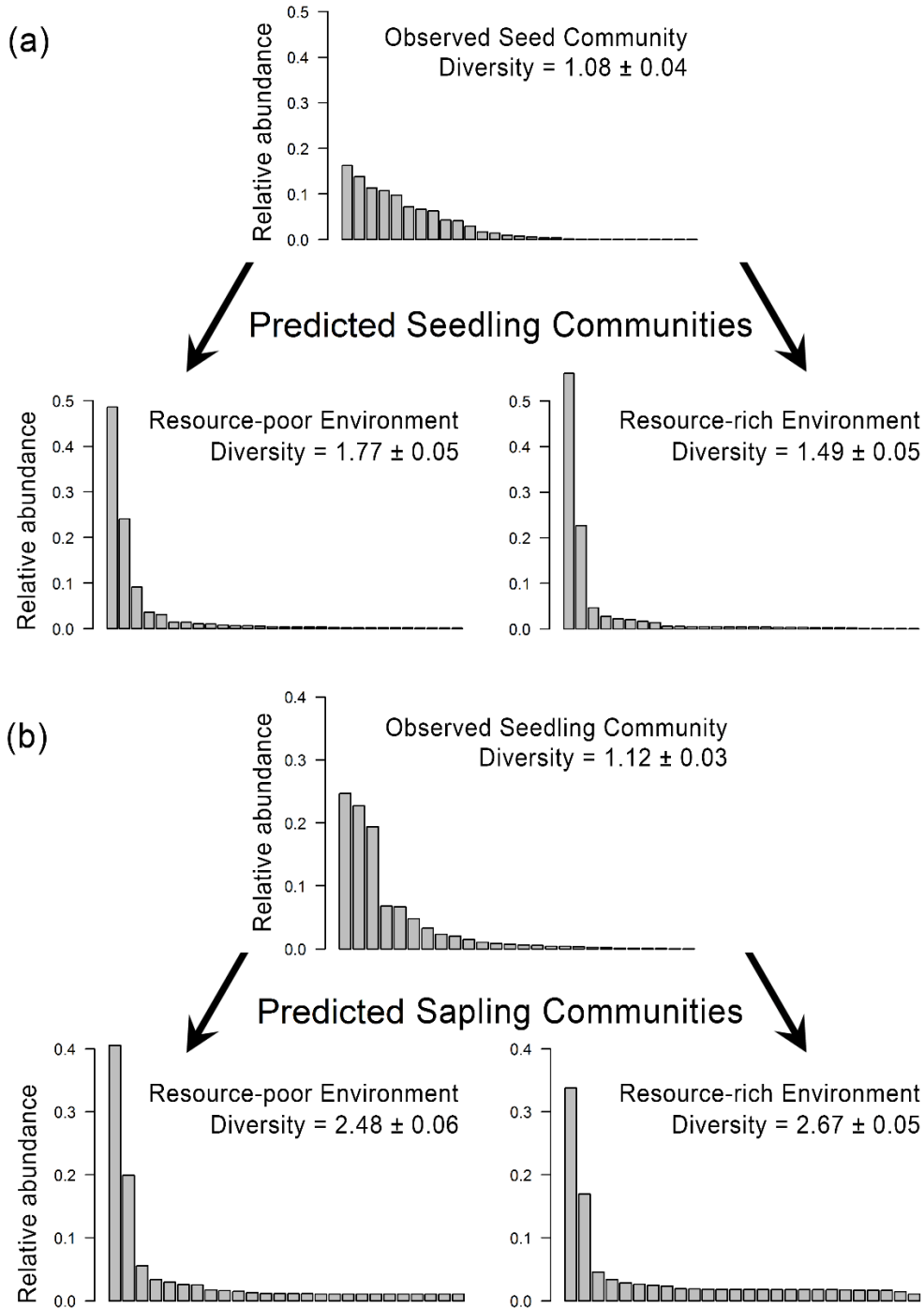
Figure S7. (a) Seedling and (b) sapling communities (species-abundance distributions) predicted from observed seed and seedling communities, respectively, using only estimated species-specific changes in negative density-dependent recruitment along the soil-resource gradient (see Fig. 2) at the Tyson Research Center Forest Plot, St. Louis, Missouri, USA. Shannon's diversity index ( \pm SE) (a) increased in resource-poor environments relative to resource-rich environments during the seed-to-seedling transition but (b) increased in resource-rich environments relative to resource-poor environments during the seedling-to-sapling transition.
