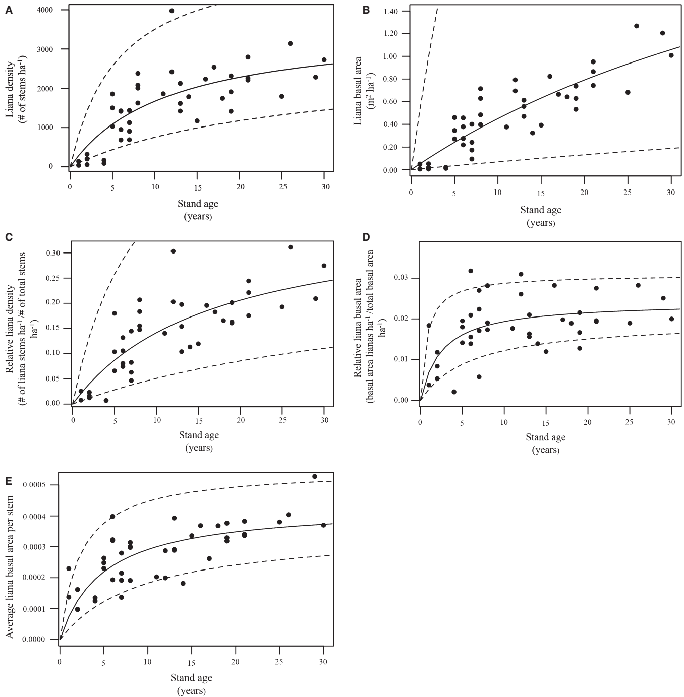
FIGURE 2. Change in liana density and basal area over forest age at Agua Salud. Liana density (A), liana basal area (B), relative liana density (# of liana stems/ha/# of total stems/ha) (C), relative liana basal area (liana basal area/ha/total basal area/ha) (D), and per stem basal area (liana basal area/ha/# of liana stems/ha) (E). All figures are for all lianas \geq 1 cm diameter. All liana metrics saturated by the time forests reached 30 yr of age, except for liana basal area (C). Solid lines represent best-fit models (Akaike information criterion Table 2) and dashed lines represent 95% confidence intervals.
