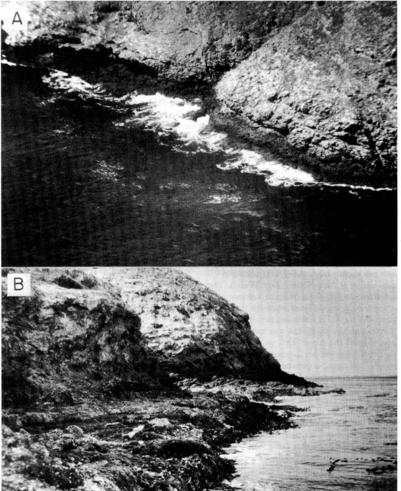
Figure 2. (A) Aerial photograph of study area on Santa Barbara Island. The diagonal indentation in the cliffs (upper center of photograph) marks Cave Canyon. (B) Northward view of shoreline at study site. Steep bluffs are located immediately shoreward of the narrow intertidal bench. The mouth of Cave Canyon is situated between the two bluffs.
