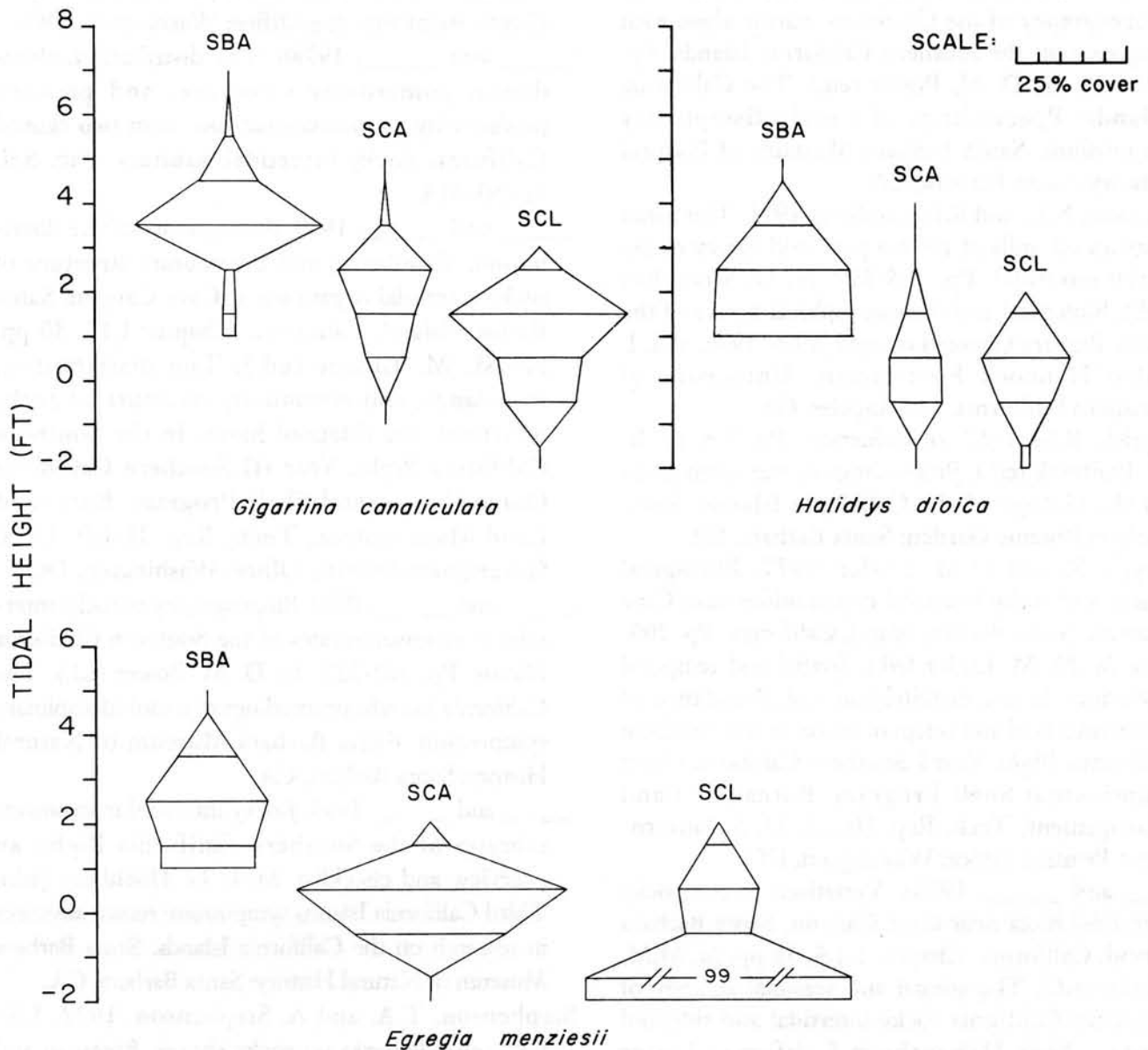
Figure 7. Comparisons of the vertical distributions (as kite diagrams of percent cover) for three species of macrophytes at Santa Barbara Island (SBA) in November 1975, Santa Catalina Island (SCA) in November 1975 and San Clemente Island (SCL) in December 1975. Mean abundance data for each 1-ft tidal interval for Santa Catalina and San Clemente Islands from Littler (1977).
