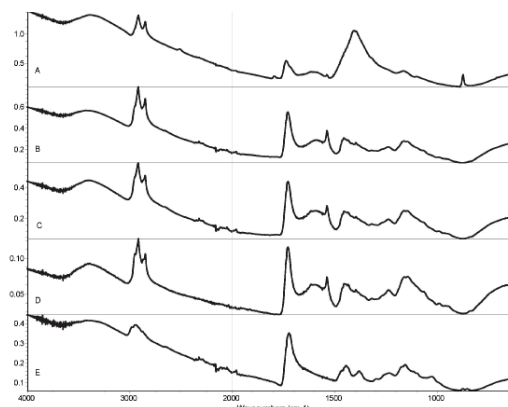
Figure 4. FTIR absorbance spectra for oil/acrylic mixtures. A: 100% oil; D: 25% oil, 75% acrylic; B: 75% oil, 25% acrylic; E: 100% acrylic; C: 50% oil, 50% acrylic;
