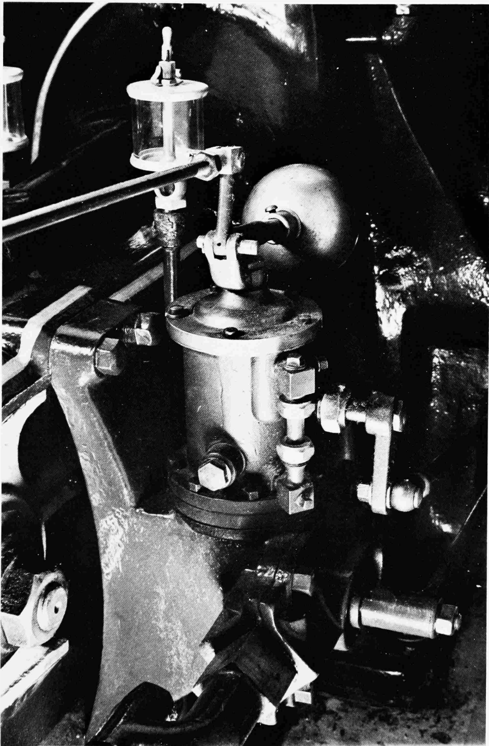
FIGURE 23.—Hydraulic governor by the "Mason Regulator Co." installed on a steam driven Frick refrigerator compressor. (NMHT 319243. Photo CLG.)
