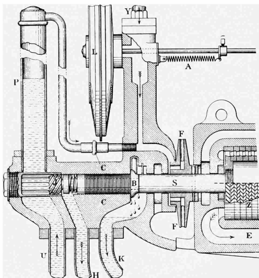
FIGURE 50.—Drawing of a Parsons steam turbine similar to NMHT 311875. Reprinted from the Proceedings of the Institution of Mechanical Engineers , 1888, pl. 85.
