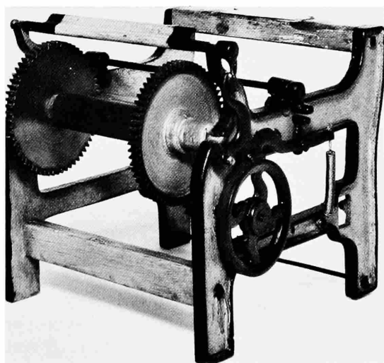
FIGURE 91.—Patent model of let-off mechanism for power looms by George Richardson, 1867. (NMHT T-11411. Smithsonian photo 71298.)
