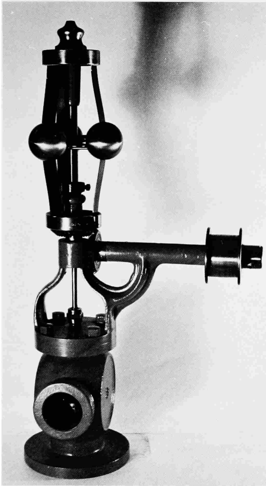
FIGURE 32.—Pickering steam engine governor, 1880s. (NMHT 310289. Photo CLG.)
