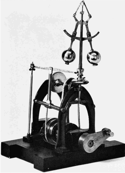
FIGURE 14.—Patent model of steam engine governor by H. A. Luttgens, 1851. (NMHT 251288. Smithsonian photo 69392.)
