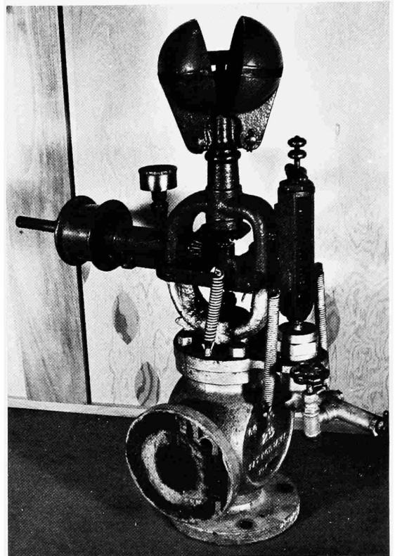
FIGURE 36.—Governor for steam-driven air compressor built by the Jarecki Mfg. Co., about 1920. (NMHT 326536. Photo CLG.)
