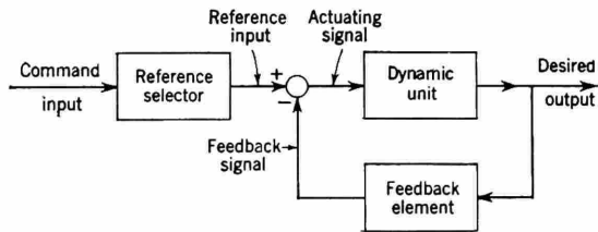
FIGURE 1.—Block diagram of a feedback control system. Reprinted from D'Azzo and Houpis, Feedback Control System Analysis and Synthesis (New York, 1960), p. 2. Used with permission of McGraw-Hill Book Company.
