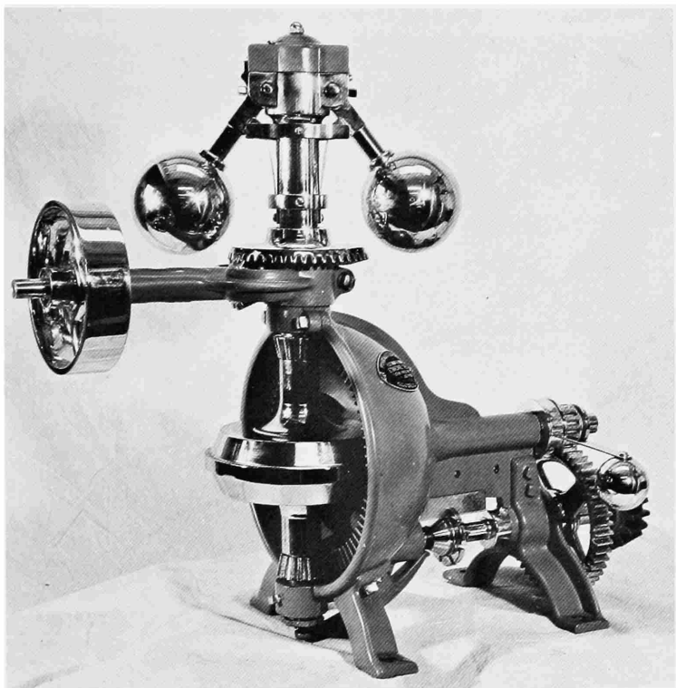
FIGURE 43a.—Woodward "Type 3" water turbine governor, 1903. (NMHT 315896, Smithsonian photo 45926-J.)
