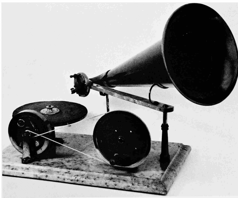
FIGURE 75.—Berliner gramophone equipped with governor (left) invented by Alfred C. Clark, 1898. (NMHT 253757. Smithsonian photo 42171-E.)
