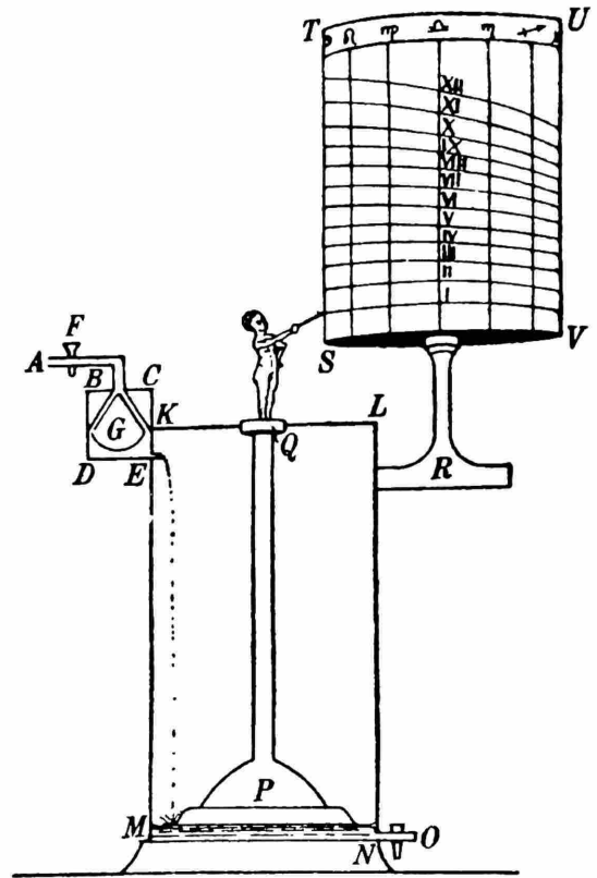
FIGURE 2.—Water clock of Ktesibios (1st half third century B.C.) as reconstructed by Hermann Diels. Reprinted from Hermann Diels, Antike Technik , 3rd edition (Leipzig, 1924), fig. 71.
