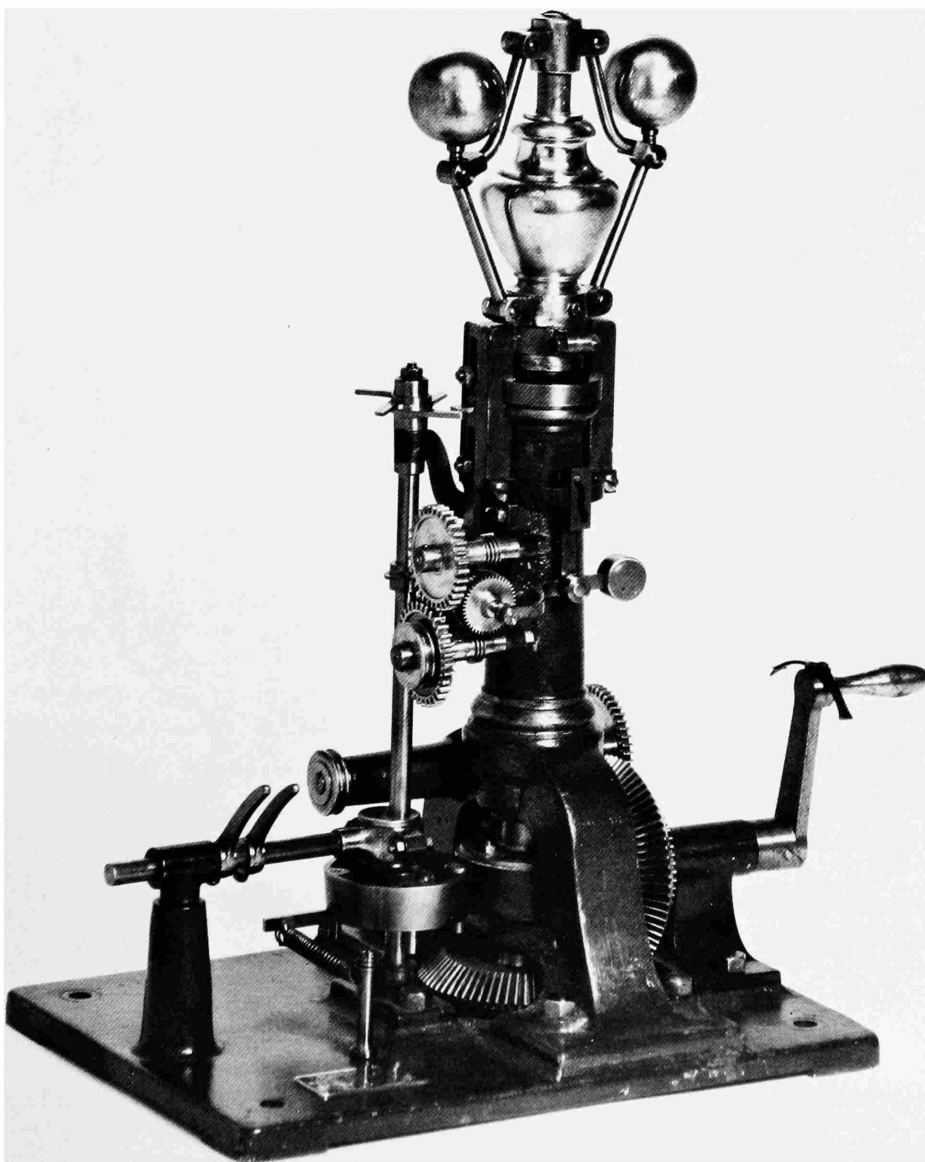
FIGURE 26.—Patent model of engine governor by Johann Georg Bodemer, 1876. (NMHT 309243. Smithsonian photo 69389.)
