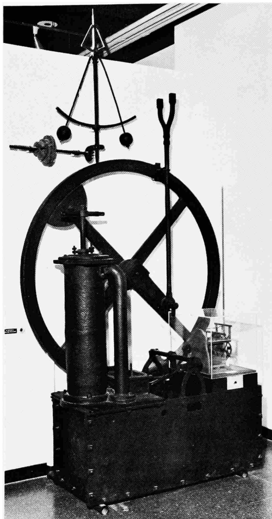
FIGURE 4.—Steam engine built in 1819 by John Holloway of Philadelphia. In the arrangement shown, the governor is not connected to the engine. Originally it was installed on the floor above the engine. (NMHT 319405. Smithsonian photo 72169.)
