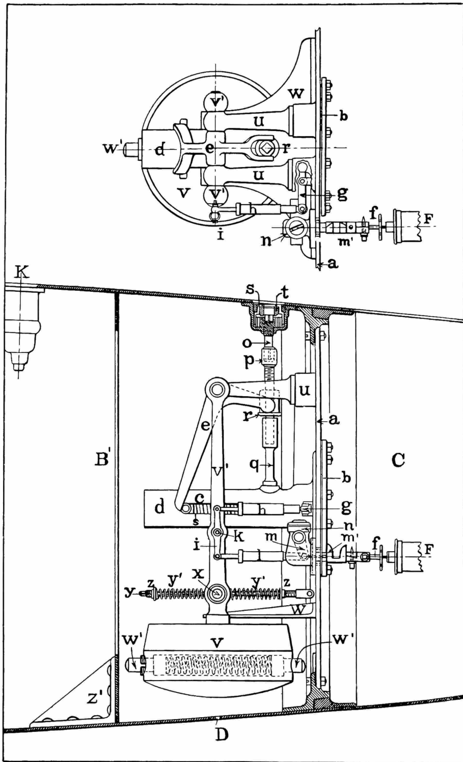
FIGURE 113.—Whitehead Mark I torpedo: the depth-control system. Reprinted from U. S. Bureau of Ordnance, The Whitehead Torpedo , 2 vols. (Washington, 1901), vol. 2, pl. 7.
