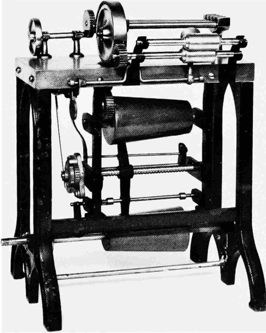
FIGURE 94.—Patent model of regulator for drawing-frames by Samuel J. Whitton, 1869. (NMHT T-11421. Smithsonian photo 71297.)
