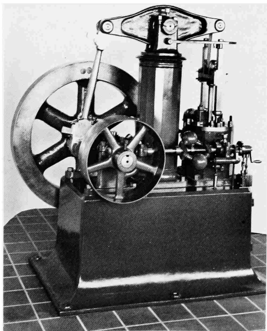
FIGURE 60.—Brayton oil engine, about 1877. (NMHT 313703. Smithsonian photo 56027.)
