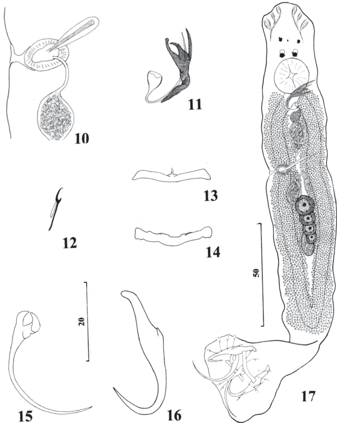
Figures. 10-17. Aristocleidus lamothei sp. n. 10, vagina. 11, copulatory complex (dorsal view). 12, hook. 13, ventral bar. 14, dorsal bar. 15, ventral anchor. 16, dorsal anchor. 17, whole mount (ventral view, haptor in dorsal view; composite). All figures are drawn to the 20 \mu scale except Fig. 17 (50 \mu ).
