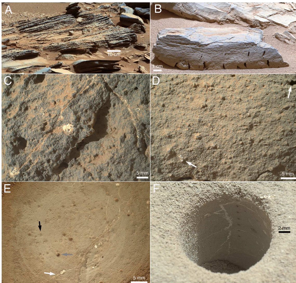
Fig. 5. Sedimentary rocks of the Yellowknife Bay formation.
