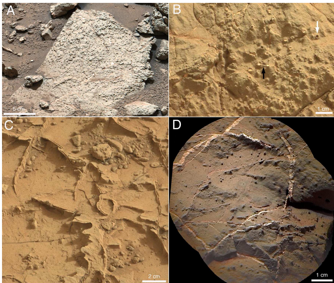
Fig. 6. Diagenetic features of the Sheepbed member.
