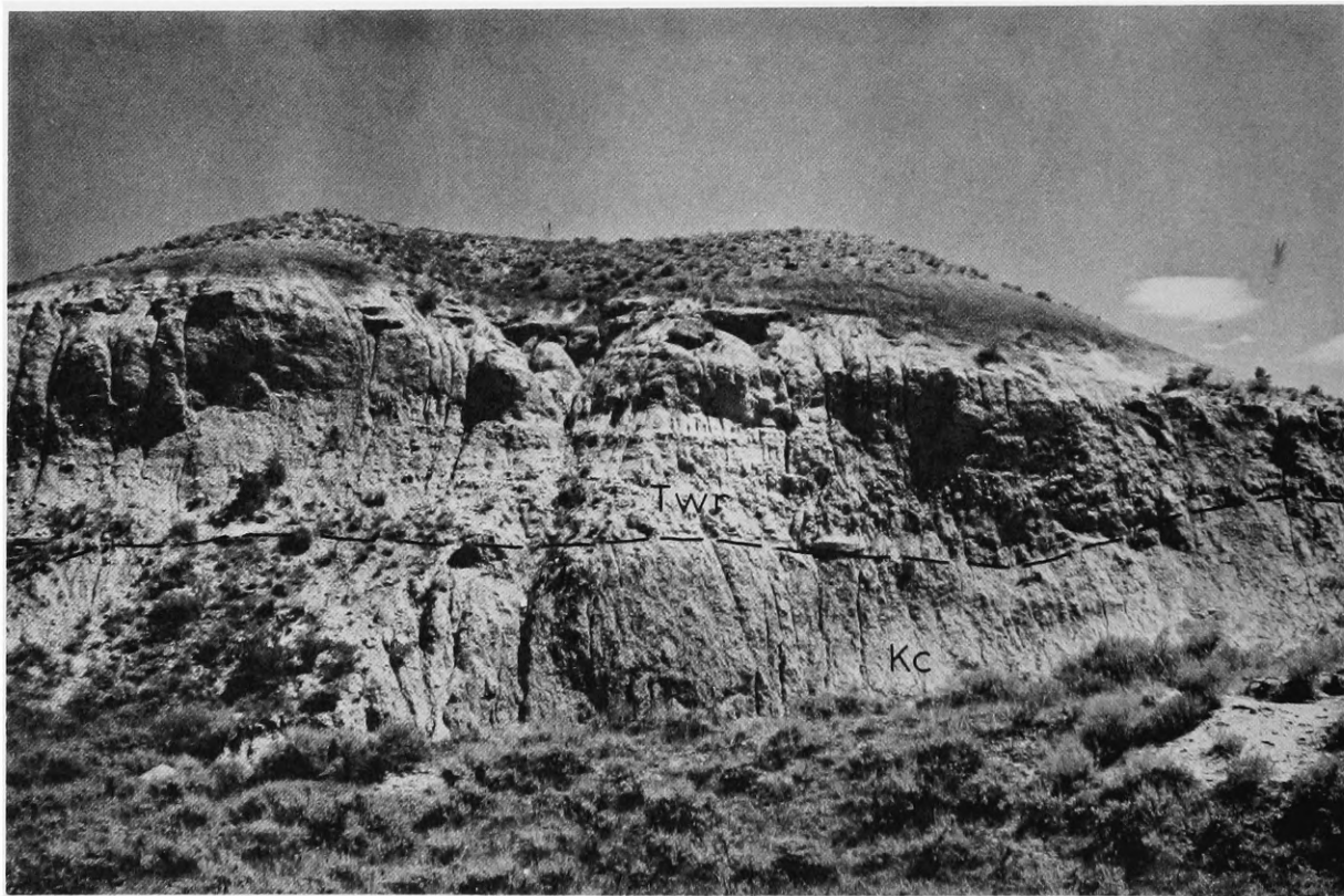
FIGURE 6. —Lower conglomeratic unit of the White River Formation (Twr) overlying Cretaceous Cody Shale (Kc) in Little Lone Tree Gulch drainage, in SE \frac{1}{4} , SE \frac{1}{4} , Sect. 13, T 31 N, R, 83 W, Natrona County, Wyoming. The basal conglomeratic unit here is up to 15 feet of cobbles of Precambrian crystalline rock and Paleozoic and Mesozoic sandstones in a coarse arkosic sandstone matrix which is locally cemented and forms ledges. This view is typical of the lower conglomeratic unit of the White River Formation over much of the Little Lone Tree Gulch drainage. The conglomeratic unit is overlain by silty bentonitic claystones of the "lower banded zone."
