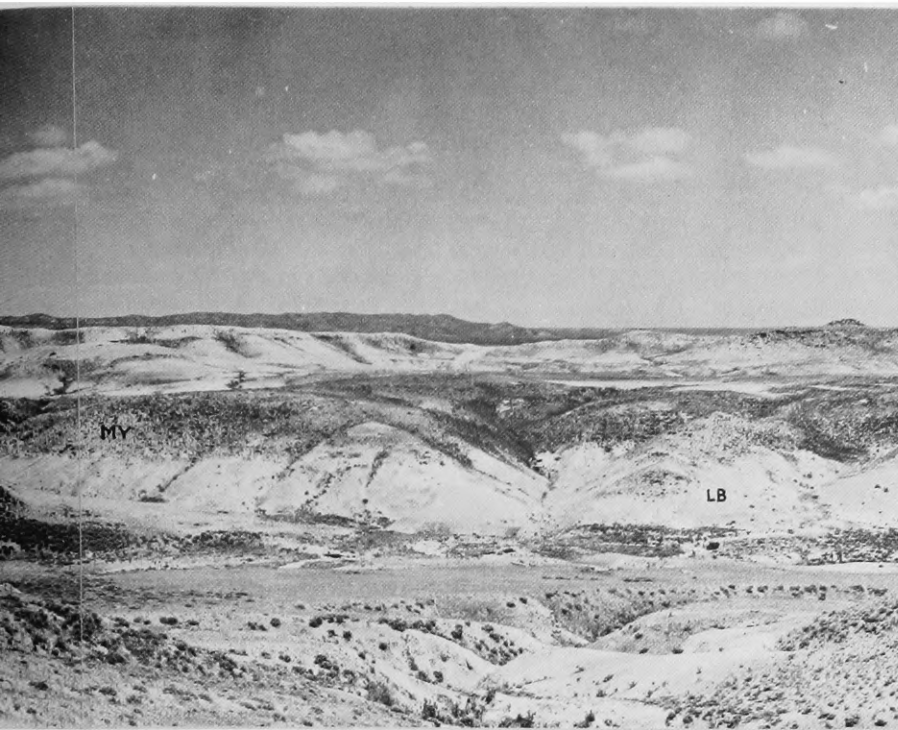
FIGURE 13.—White River Formation in Little Lone Tree Gulch. View generally northwestward with north-east end of Flagstaff Rim at left. Letter symbols indicate units discussed in text: LB = “lower banded zone,” MY = “middle yellow sandstones,” UB = “upper banded zone,” B indicates approximate position of volcanic ash B.
