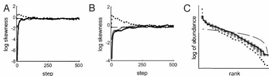
Fig. 3. Convergence of the shape of the SAD. (A and B) Convergent series of skewnesses of 5ADs- p of log-transformed abundances starting with left-skewed (bold line), regular (thin line), and right skewed (dotted line) initial-SADs- p . Each series is parameterized by species spatial turnover and spatial autocorrelation of (A) tropical tree and (B) central European bird data. Dashed lines show the observed skewnesses. (C) Rank-log-abundance plots of the central European bird data (thin line), and a result of the respective convergent series (gray circles; steps 300–500), which started as the regular initial-SADs- p (dashed). For contrast see the tropical tree data (dotted line). SADs are standardized (mean abundance = 1), and veiled by minimum observed values.
