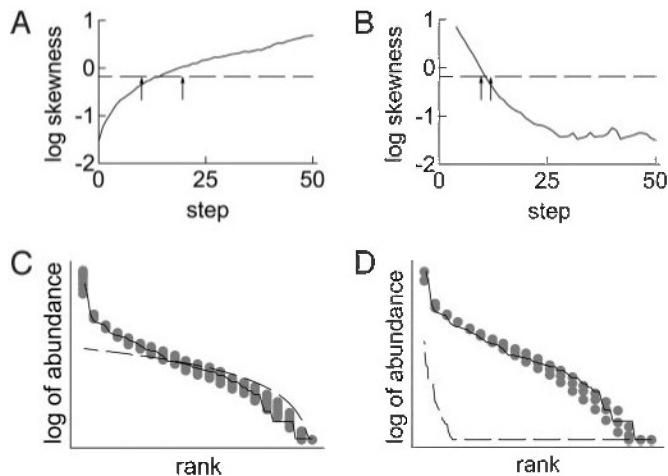
Fig. 4. Simulated series of skewnesses of 5ADs- p of log-transformed data starting with (A) regular and (B) right-skewed initial-5ADs- p and Central European bird data for 1/8 of the transect. The observed value (dashed line) is crossed in between steps 10 and 20 in A, and 10 and 12 in B (spaces between arrows). The simulated rank-log-abundance plots for these steps (gray circles) are plotted in C and D, respectively. Observed 5AD p is marked by a solid line, initial-5ADs- p s are dashed. Series vary in their parameters (for settings see Materials and Methods ), but their values have little effect on the agreement between data and simulations ( SI Appendix , Fig. S2).
