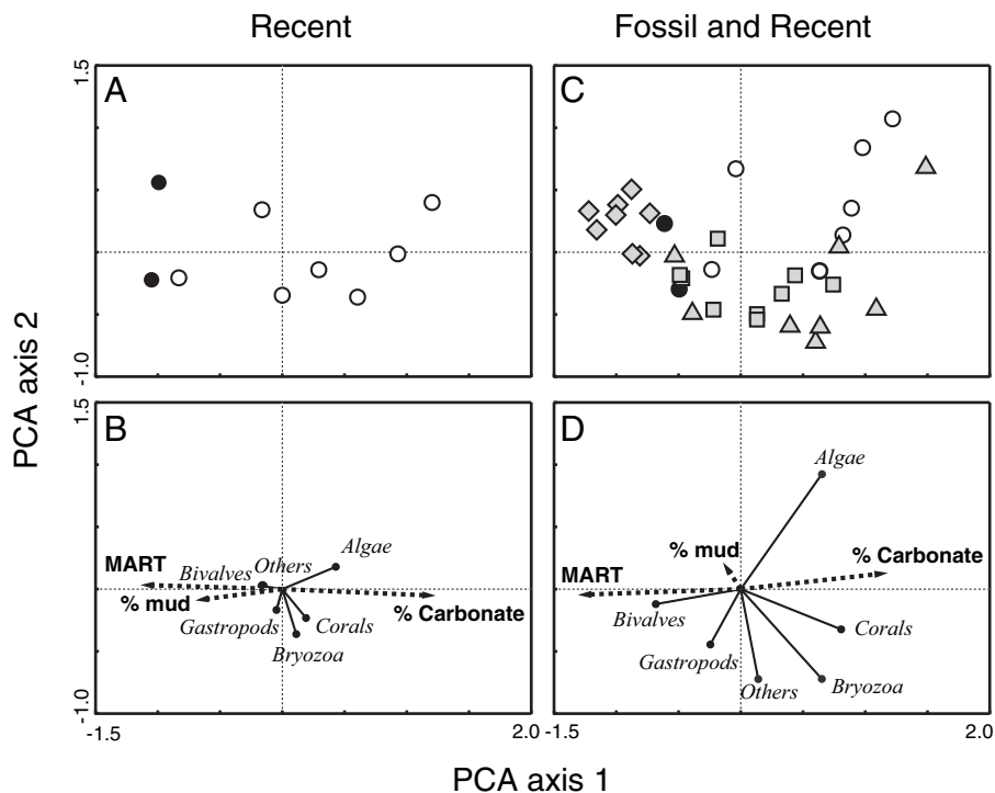
Fig. 2. Ecological structure of Central American Recent (Left) and fossil and Recent faunules (Right). (A) Ordination of Caribbean recent faunules based on biotic composition. (B) Taxa and environmental variables that best explain the ordination. PCA axis 1 describes a gradient from predominantly heterotrophic bivalves to mixotrophic corals that closely correlates with carbonate production and mean annual range of temperature (MART). (C) Adding the fossil Caribbean faunules to the ordination produces a similar pattern with scores of most fossil faunules intermediate between those for Recent Caribbean and Pacific faunules that again (D), reflects the opposite distributions of bivalves and corals correlated with MART and % carbonate. In B and D, solid lines with terminal spots are ordinations for different taxa. Dashed lines with arrows are environmental correlations that best explain the ecological variation observed. See Fig. 1 for legend.
