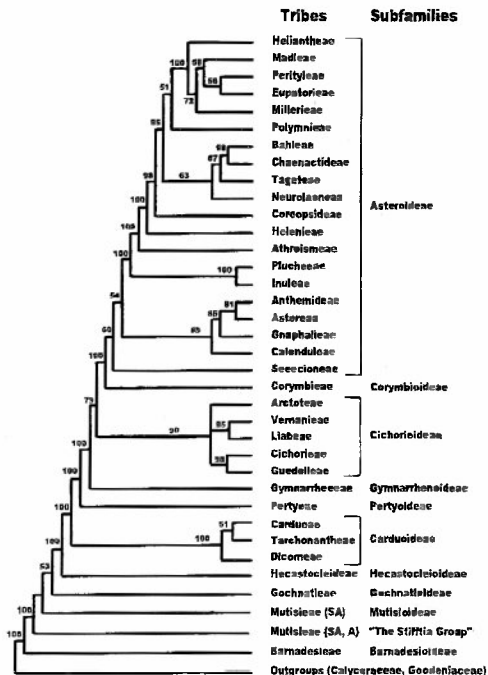
Fig. 1. Strict consensus tree of 12 most parsimonious trees for 122 representative Compositae taxa based on chloroplast DNA sequence data. Bootstrap values indicated above nodes, SA = South America, A = Asia. Tree is simplified to show only tribe and subfamily placement and arrangement.
