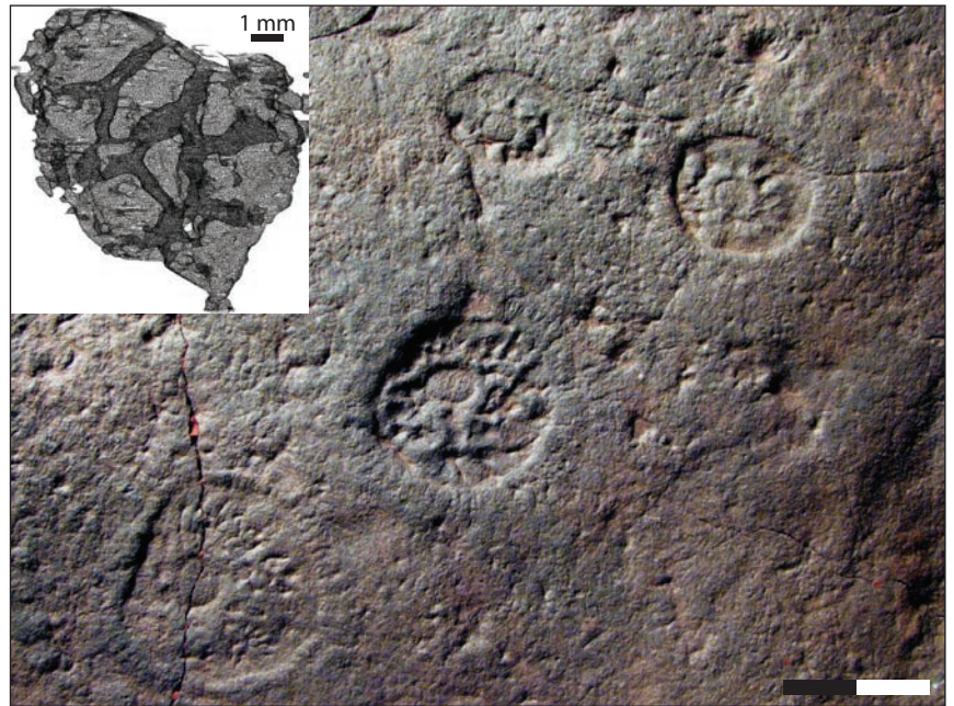
Figure 1 | The earliest probable sponges include the Ediacaran Paleophragmodictya (SAM P32352A-F), found in the Flinders Ranges of South Australia. Maloof and colleagues 6 describe fossils from older sections in the Flinders Ranges (inset). These globular, asymmetric forms have unusually large networks of canals and are interpreted as the remains of primitive sponges that lived 90 Myr earlier than Paleophragmodictya . Scale bar: 2 cm.
