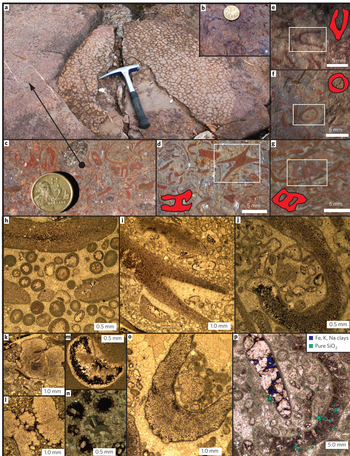
Figure 2 | Diverse morphology of the Trezona Formation fossils. a–g. Outcrop photographs from the Trezona Fm showing the range of skeletal morphologies in fossil debris onlapping and draping a stromatolite bioherm (under the hammer in a ). b depicts tabular beige stromatolite flake breccia in the lower left mixing with distinctive red fossil debris in the upper right. For each 3D model presented in Fig. 3, we extracted 624 2D sections to compare to the common 2D sections apparent in outcrop (Supplementary Fig. S4). Common shapes in both outcrop (photos) and in 2D sections through the models (red objects) include anvils ( d ), wishbones ( e ), rings ( f ) and perforated slabs ( g ). h–p. Thin-section photomicrographs in plane polarized light. The matrix in all samples is composed of equant interlocking calcite crystals. Floating in the matrix are 0.1–0.5-mm-diameter spherical ( h,n ) and kidney-shaped ( m ) grains composed of crystalline calcite interiors with variable quantities of opaque clay, and extremely fine micritic calcite coatings ( h ). Bioclasts are a mix of opaque clays (dark blue in E-SEM EDXs element map overlay on transmitted and reflected light photomicrograph (in p )), 0.05–0.1 mm pure SiO 2 blebs (green in E-SEM EDXs overlay (in p )) and calcite crystals that sometimes coarsen towards the edges of the clasts ( j ). In general, wishbones tend to have the distinctive SiO 2 blebs (lower right of p ), anvils contain more uniformly micro-crystalline calcite with disseminated SiO 2 and tabular flakes tend to have coarser calcite interiors with larger clay patches (upper left of p ). Bioclast edges have micritic rims irrespective of the interior crystal size. k and l depict bulbous, chambered micro-textures similar to polymuds reported from other Neoproterozoic microbialites 37,38 .
