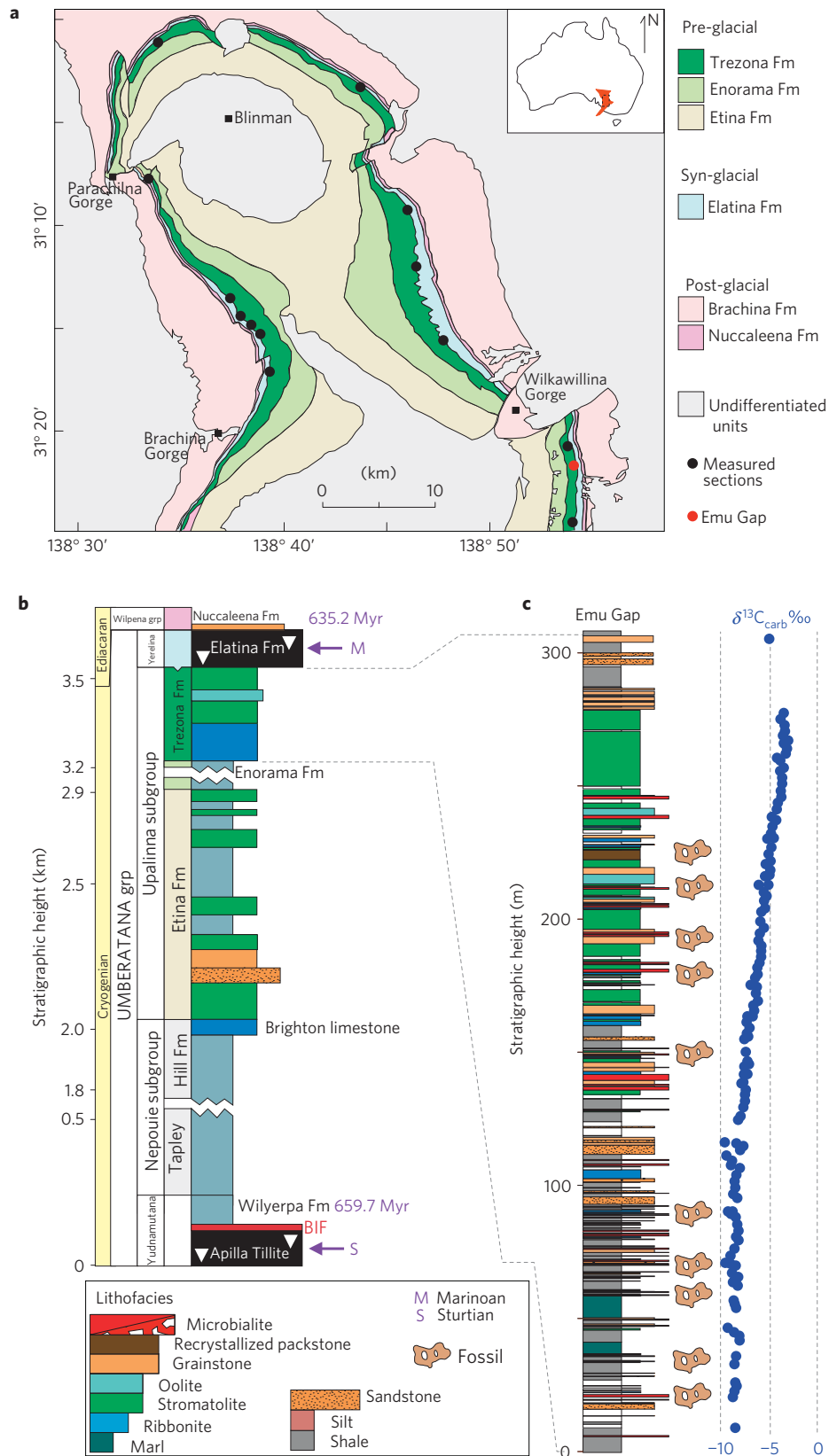
Figure 1 | Geological and stratigraphic setting of the Trezona Formation. a , Geological map of the central Flinders Ranges, with measured section locations marked by black and red dots. The Australia map inset locates the Adelaide Rift Complex in red and the central Flinders study region in the dashed black rectangle. b , Schematic stratigraphic section through the Cryogenian of South Australia. Note the changes in scale within the thick Tapley Hills and Enorama Fm siltstones. The 635.2 Myr age for the end of the Marinoan ice age comes from correlation to Namibia 8 and China 7 . The 659.7 Myr age for the Wilyerpa Fm comes from a section in the northern Flinders 2 . c , Detailed lithostratigraphy and \delta^{13}\text{C}_{\text{carb}} from Emu Gap, with labelled fossil horizons. Etina Fm carbonates have near-constant \delta^{13}\text{C} values of +8‰ (ref. 45).
