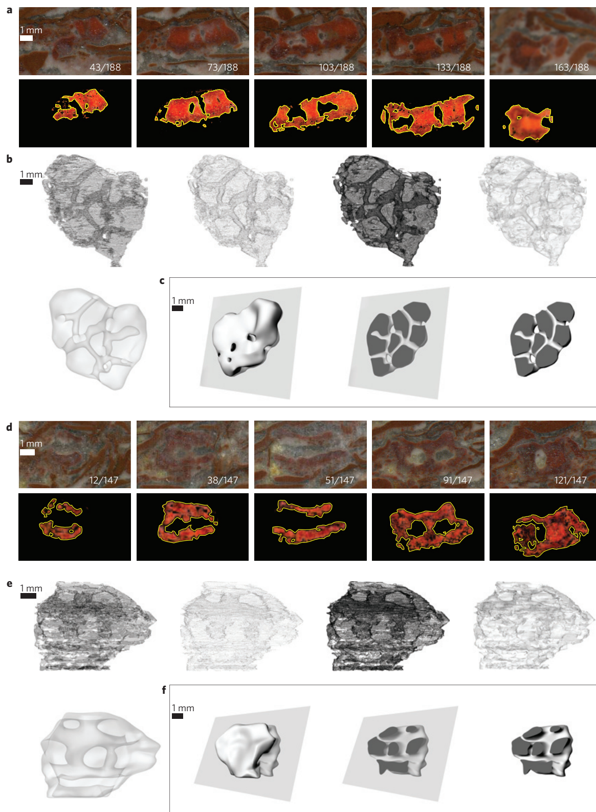
Figure 3 | Three-dimensional reconstruction of the Trezona Formation fossils. a–f , Digital models of two specimens ( a–c and d–f ). a,d illustrate the auto-trace (yellow lines) routine in 5 (of 188 and 147) serial images used to construct the model in b,c and e,f . The top panel of a,d contains raw images with white labels indicating the frame number of each section, and the bottom panel of a,d contains contrast-enhanced images with yellow auto-traces. b,e depict, from left to right, the original auto-traced polygons arrayed in the third dimension, the polygons converted to a point cloud, the raw mesh derived from the point cloud, a semi-transparent 3D model volume of the mesh and a low-pass-filtered version of the semi-transparent model. c,f is a rendered depiction of the smooth model volume, then sliced perpendicular to the plane of the original traces in a,d . These specimens are asymmetric, both in its external form and internal canal network, although the canals are of uniform diameter. The specimens in a–c and d–f are representative of the external and internal topologies found in the best preserved fossils.
