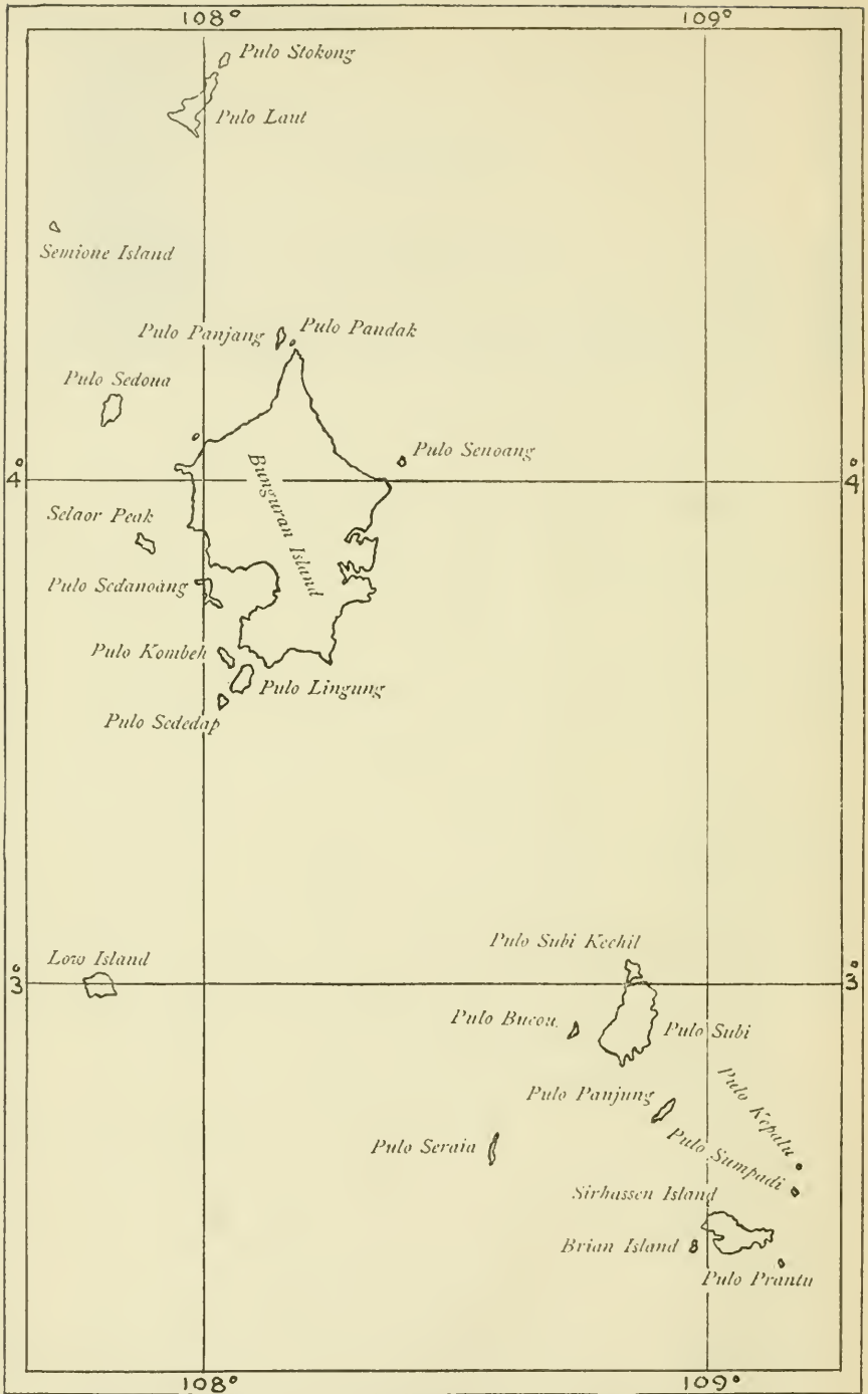
FIGURE 1.—The most important islands of the Natuna Group, South China Sea.
